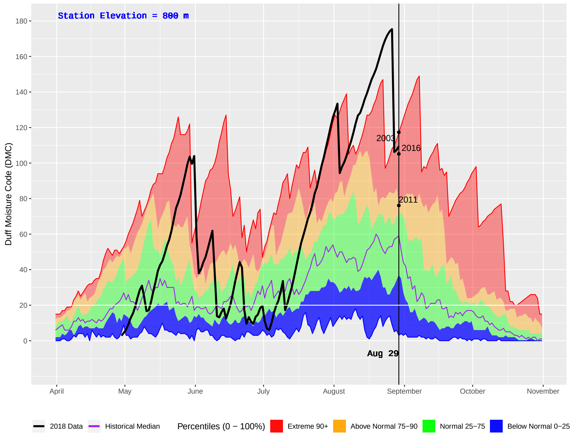
GOLD HILL (379) : Historical (1979–2016) and Current (2018) Daily Duff Moisture Code (DMC)
