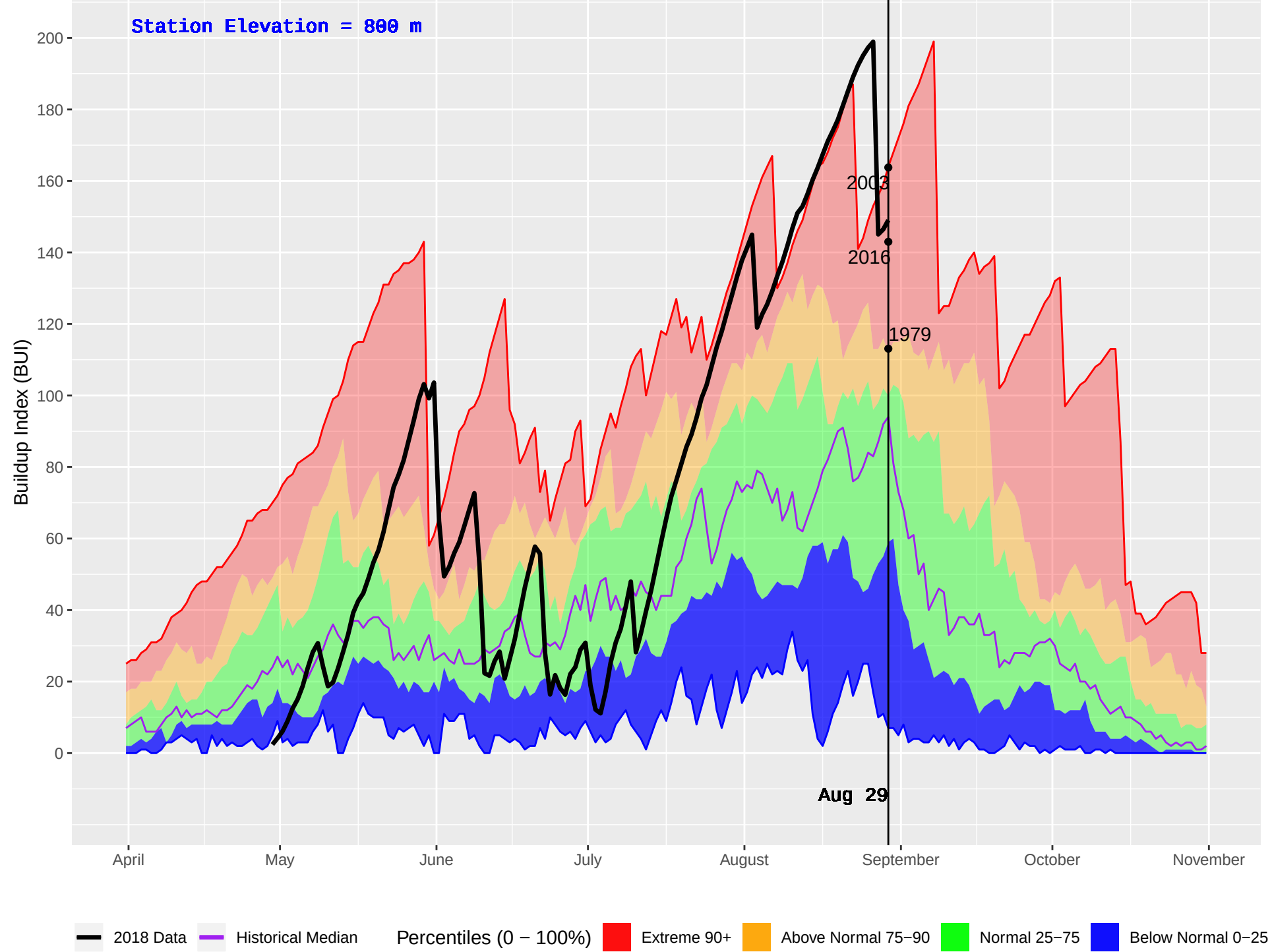
GOLD HILL (379) : Historical (1979–2016) and Current (2018) Daily Buildup Index (BUI)
