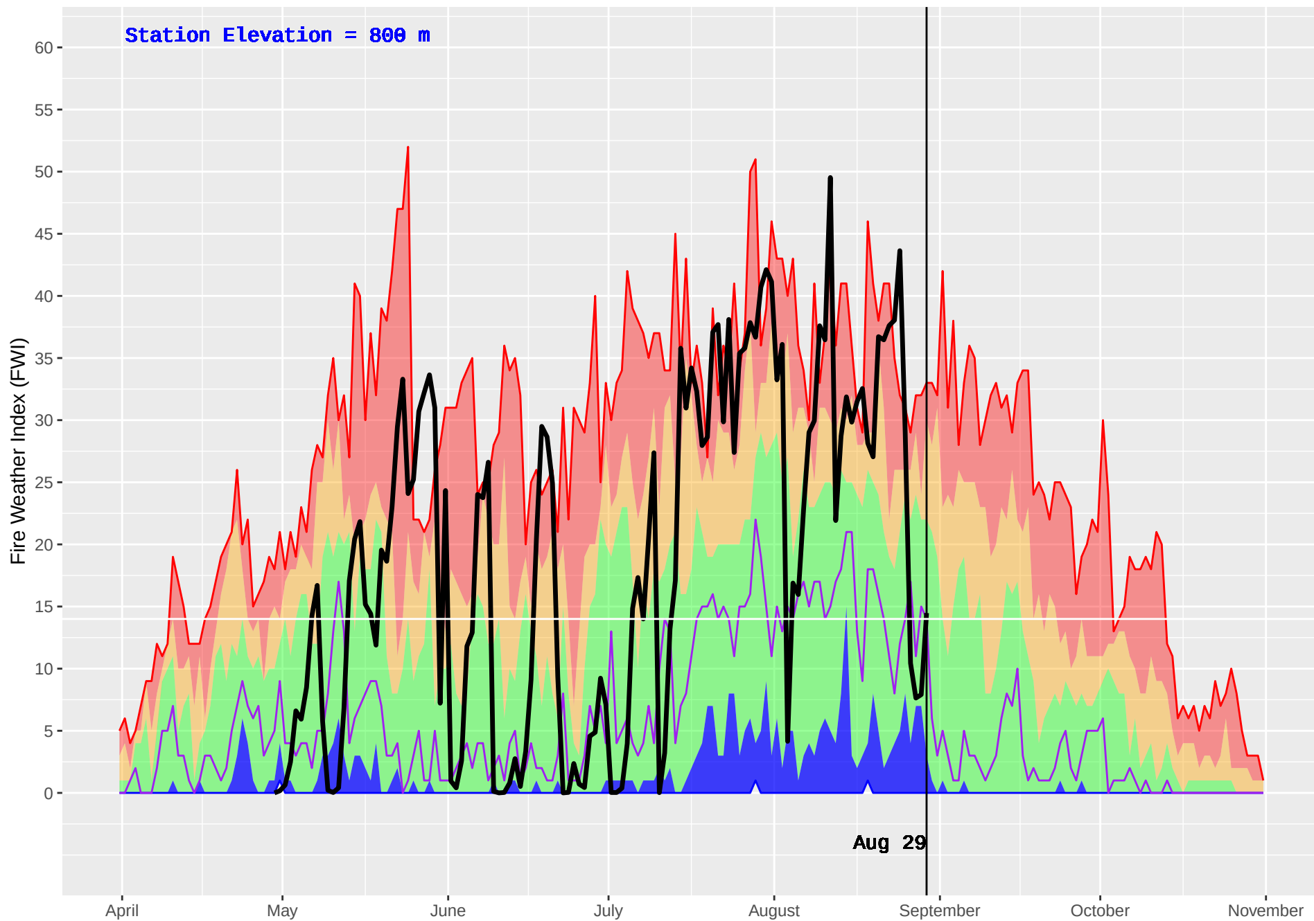
GOLD HILL (379) : Historical (1979–2016) and Current (2018) Daily Fire Weather Index (FWI)
