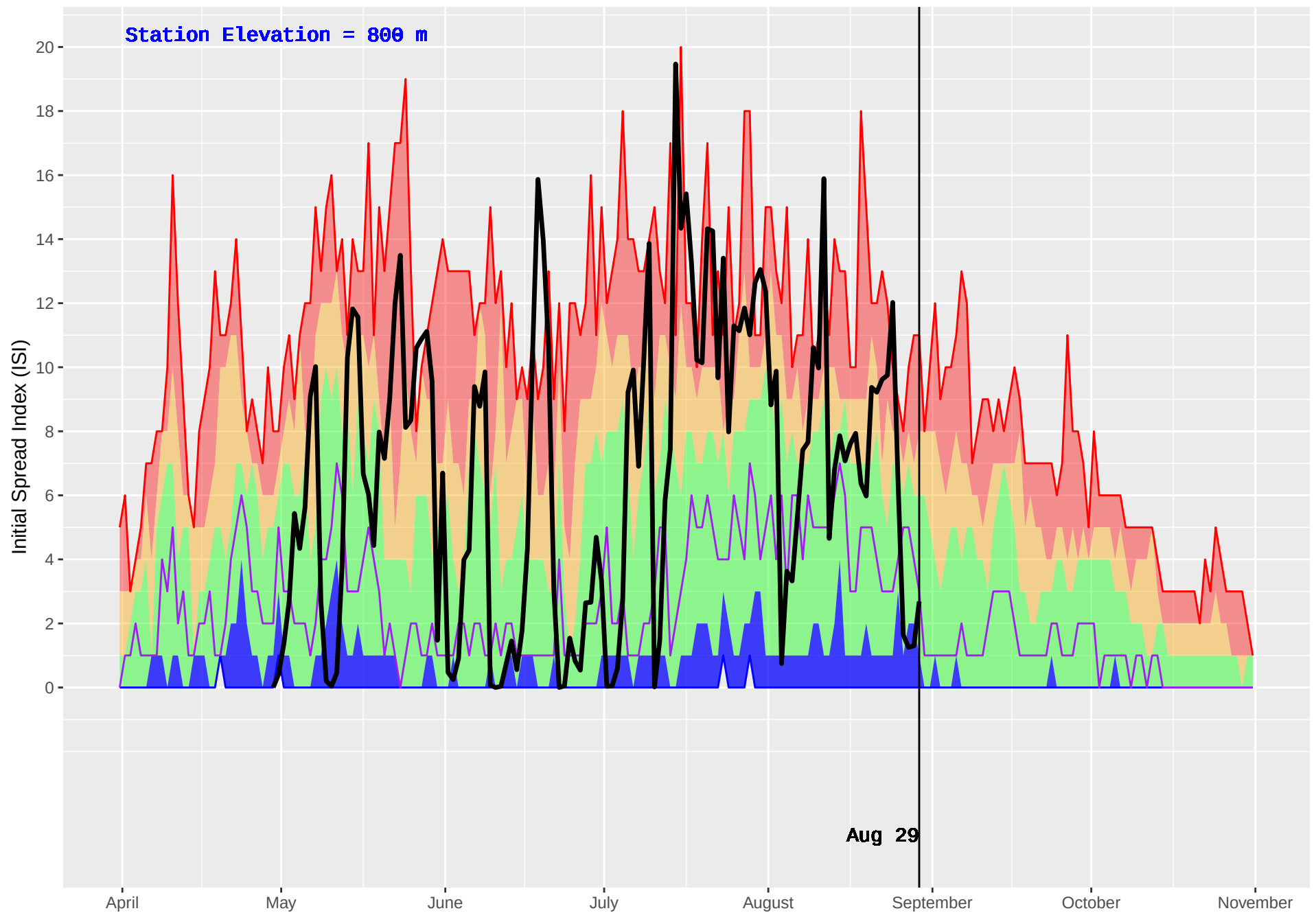
GOLD HILL (379) : Historical (1979–2016) and Current (2018) Daily Initial Spread Index (ISI)
